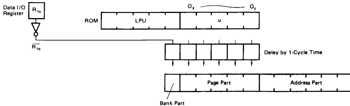
Figure 7 LPU Operation
