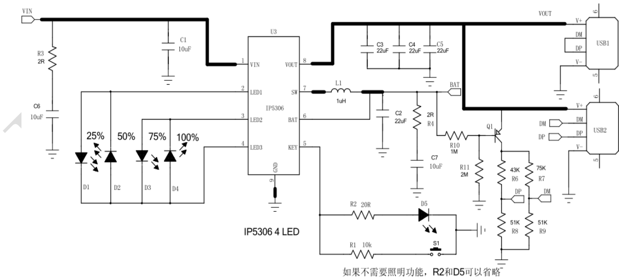
图 7 4 LEDs SOC indicator typical application schematic
