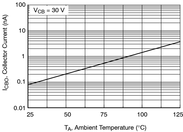
Figure 5. Collector Cut-Off Current vs. Ambient Temperature
